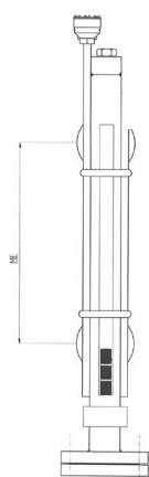
Mounted at a Bypass-pipe Design for insulation type 745.200X
